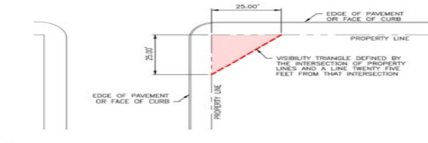
Figure. 6.1 Visibility Triangle
